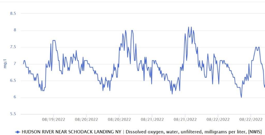
HRECOS Analysis
